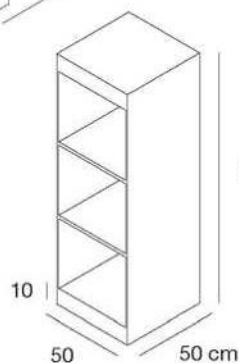
2M01/N Modulo vani nobilitato Compartment module faced panel L50 x P50 x H150 cm
