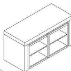
2T02/N modulo vani con ruote nobilitato compartment with wheels faced panel L35 x P65 x H70 cm
